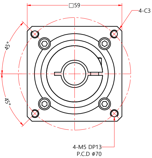
VIEW A
