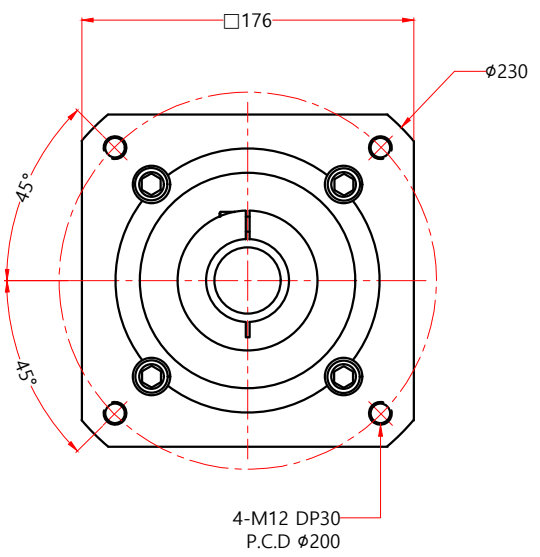
VIEW A
