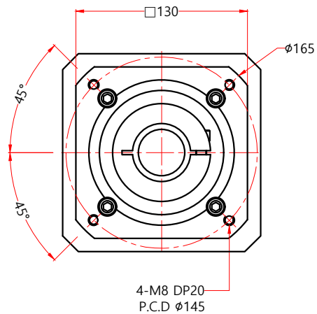
VIEW A
